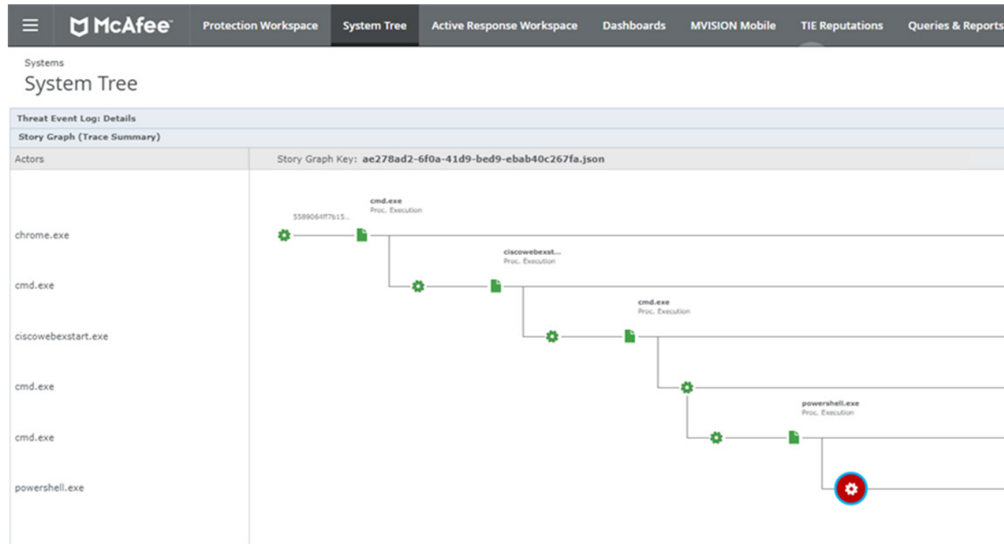
Figure 1. Story Graph.
